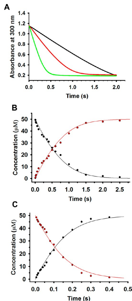
Figure 6. (A) Time courses for the hydrolysis of 100 \mu\text{M} 4-hydroxybenzoyl-CoA catalyzed by 10 \mu\text{M} (green), 16 \mu\text{M} (red), and 20 \mu\text{M} (black) YdiI in 50 mM \text{K}^+\text{HEPES} (pH 7.5) at 25 ^\circ\text{C} . Reactions were monitored at 300 nm using a stopped-flow spectrophotometer. (B) Time course for the YdiI (20 \mu\text{M} )-catalyzed hydrolysis of 50 \mu\text{M} [ ^{14}\text{C} ]-benzoyl-CoA in 50 mM \text{K}^+\text{HEPES} (pH 7.5) at 25 ^\circ\text{C} ; (black filled circles) concentration of [ ^{14}\text{C} ]-benzoyl-CoA and (red filled circles) concentration of mixed [ ^{14}\text{C} ]-labeled anhydride intermediate and/or [ ^{14}\text{C} ]-benzoate remaining in reaction solution upon the acid quench. (C) Same as in (B) except that 4 \mu\text{M} YdiI and 50 \mu\text{M} [ ^{14}\text{C} ]-benzoyl-CoA were used.
